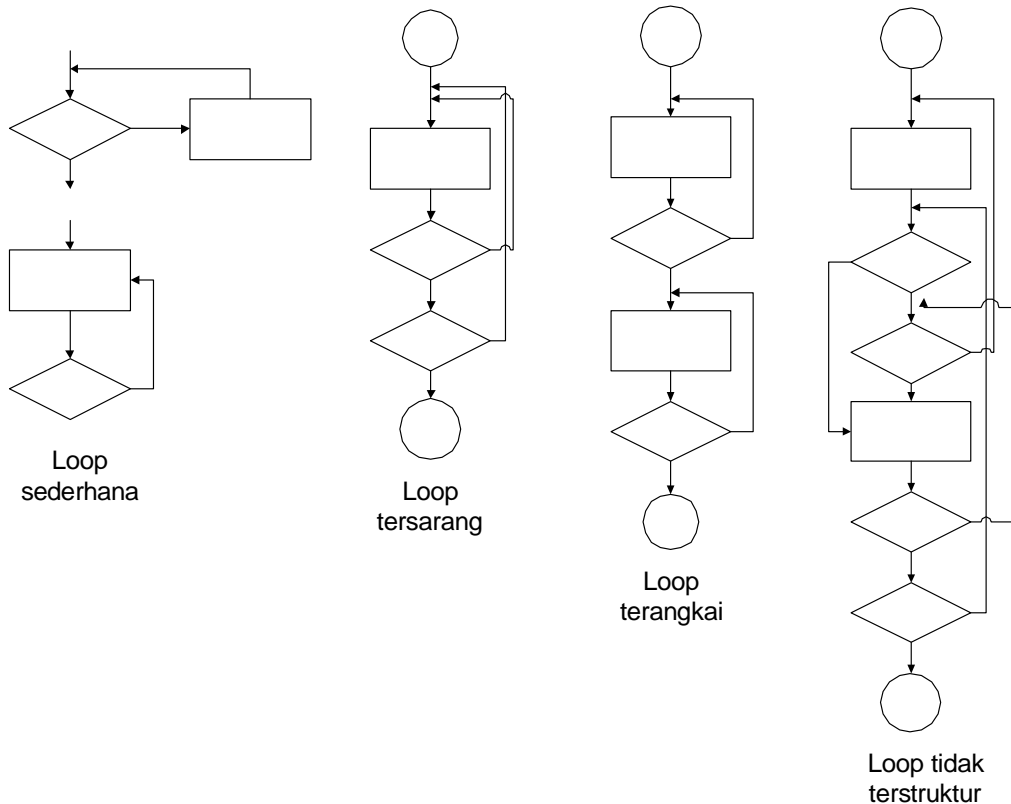
Gambar 9.9. Macam-macam loop
